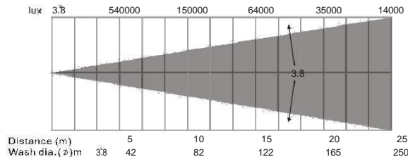
PHOTOMETRICS DIAGRAM 3:8
